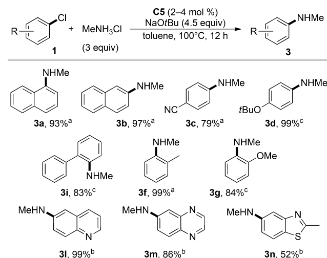
Scheme 2. Nickel-catalyzed amination of aryl chlorides with methylamine hydrochloride. Reactions were performed with 0.60 mmol of the aryl chloride. Yields of isolated products are given. [a] 2 mol% C 5 . [b] 3 mol% C 5 . [c] 4 mol% C 5 .
